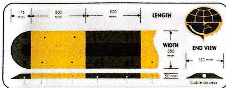
Gambar 1 Speed Bump
